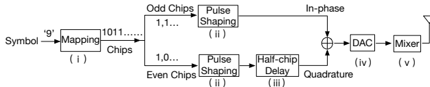
Fig. 2. ZigBee transmitter
