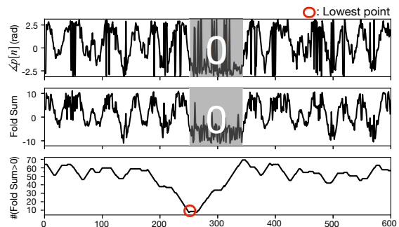
Fig. 11. SymBee preamble detection success example (SNR=-10dB)
