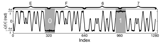
Fig. 7. Phase ( \angle p[n] ) of SymBee signal in practice, when bits 0 and 1 are sent back to back. Gray region indicate corresponding stable phase.
