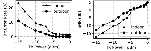
(a) BER under different power level. (b) SNR under different power level. Fig. 19. Impact of transmission power.
