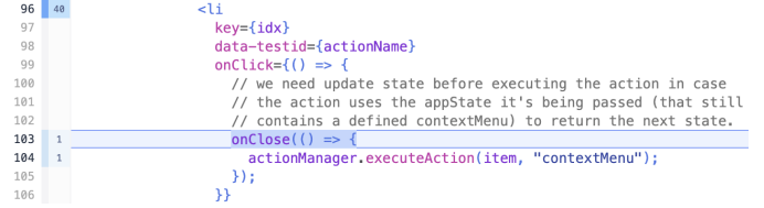
Fig. 6. The jump to code target of Bugs 2 and 3
