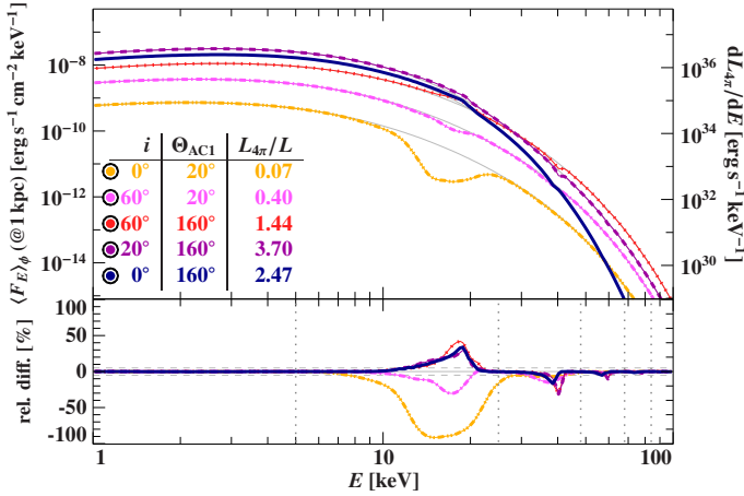
Fig. 8. Phase-averaged spectra of a single accretion column in the observer frame. Each spectrum corresponds to a different setup ( i , \Theta_{AC} ) indicated in the table inlet. Solid gray lines correspond to the case without CRSFs. The bottom panel shows the relative difference of the spectra to their pure continuum contribution, where horizontal dashed gray lines mark \pm 5\% . CRSFs energy ranges are indicated with the vertical dotted gray lines.
