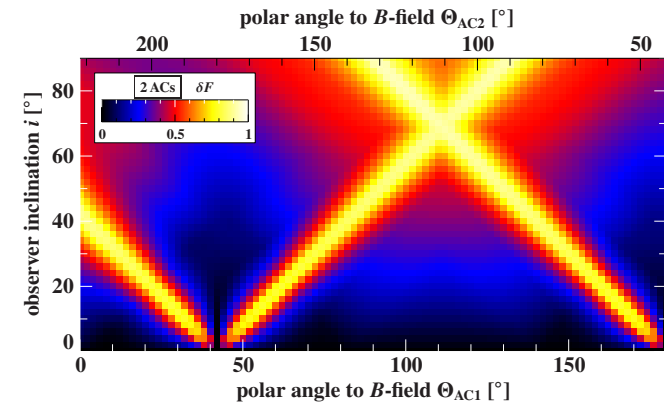
Fig. A.2. Pulsed fraction of energy-integrated pulse profiles for the asymmetric setup.
