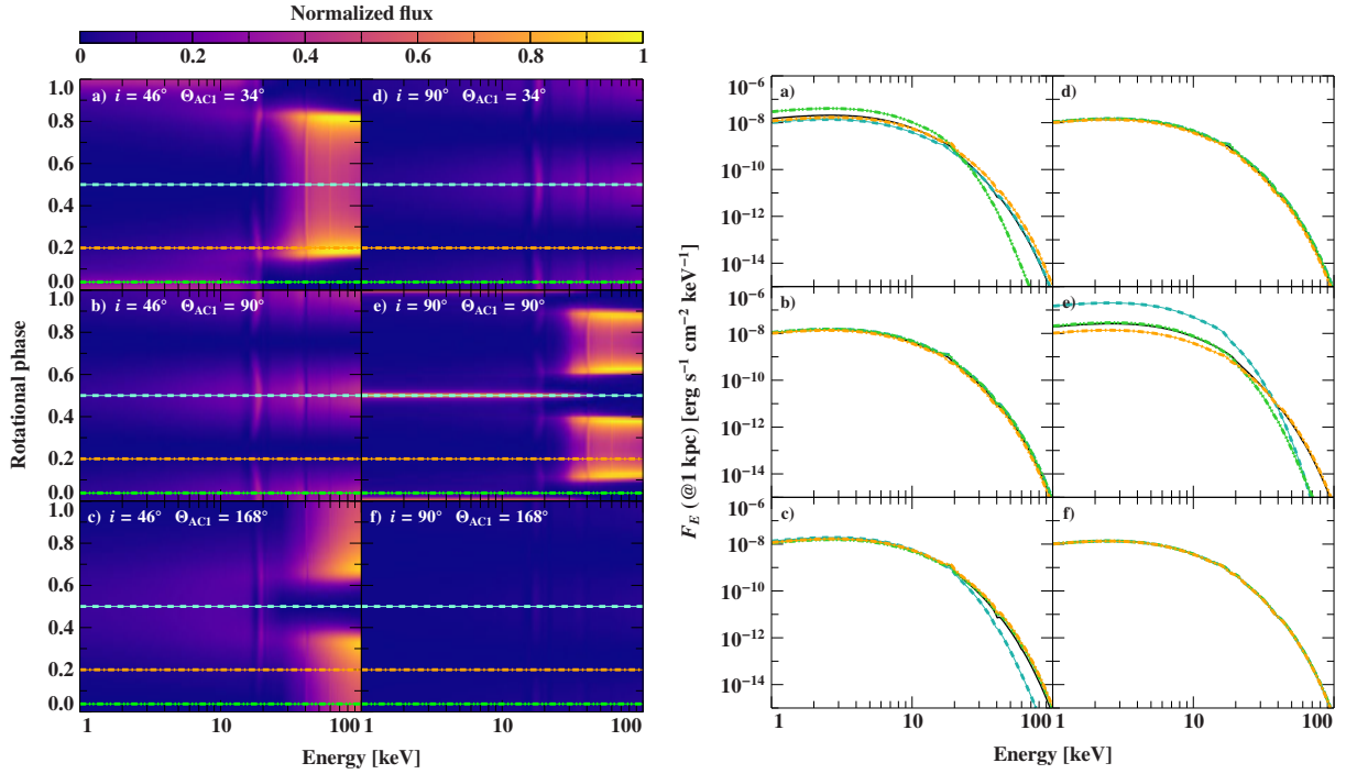
Fig. 11. Same as in Fig. 10, but for different antipodal column geometries ( i, \Theta_{ACI,2} ).
