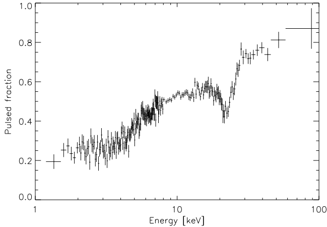
Fig. 2. Pulsed fraction as function of energy, from 1.2 to 8 keV the data are from MECS, from 8 to 30 keV from HPGSPC , and from 30 to 120 keV from PDS .
