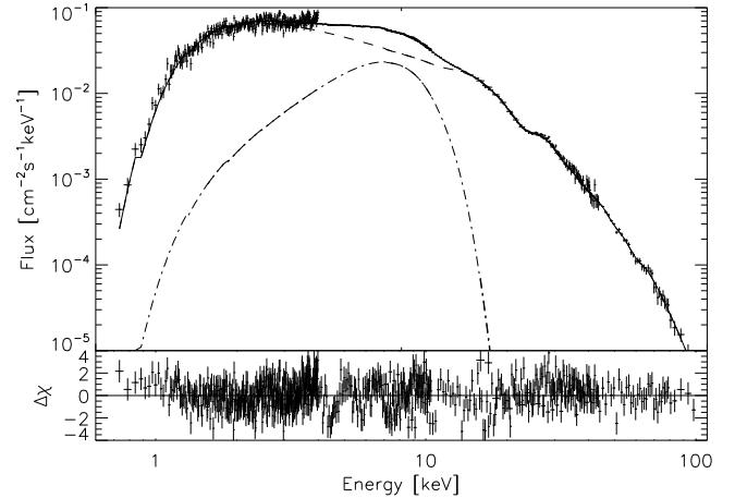
Fig. 3. Upper panel: the unfolded spectrum of 4U 0115+63 described by the phenomenological model: the dashed line is the high-energy cut-off power law, the dot-dashed line the broad Gaussian, and the solid line the sum. The spectra of the four instruments have been scaled according to the inter-calibration constants of Table 1. Lower panel: residuals from the best fit model.
