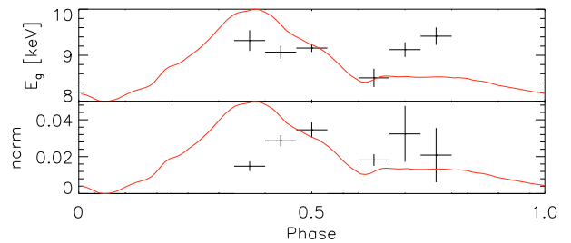
Fig. 8. Best fit parameters for the Gaussian emission line as function of the phase. The line width is fixed to 1 keV. The solid line is the smoothed pulse profile in the 10–20 keV energy band with arbitrary normalization.
