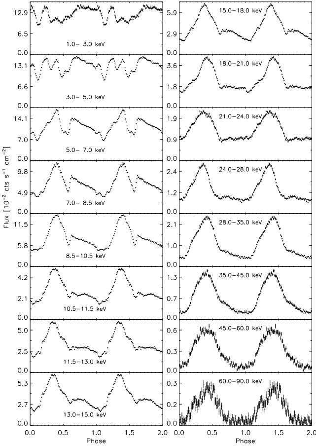
Fig. 1. Pulse profiles of 4U 0115+63 in different energy ranges. The data are from the MECS (1.0–8.5 keV), HPGSPC (8.5–28 keV) and PDS (28–95 keV) instruments on board of BeppoSAX .
