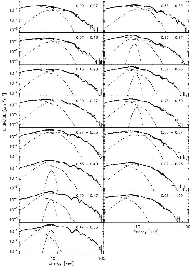
Fig. 5. Unfolded phase resolved spectra. The phase range is indicated in each plot. The dashed line is the thermal Comptonization, the dot-dashed line the column emission computed using the BW model, the dot-dot-dashed line a narrow Gaussian line, and the solid line the sum.
