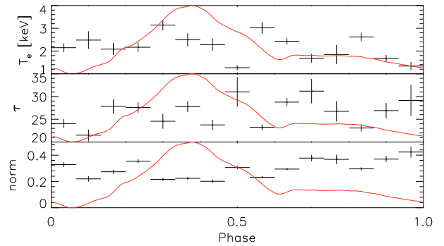
Fig. 7. Best fit parameters for the soft Comptonization spectral component (compTT) as function of the phase. The temperature of the seed photons is fixed to 0.51 keV. The solid line is the smoothed pulse profile in the 10–20 keV energy band with arbitrary normalization.
