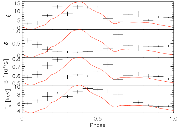
Fig. 6. Best fit parameters for the Becker and Wolff spectral component as function of the phase. The accretion column radius is fixed at 600 m and the mass accretion rate at 6 \times 10^{16} \text{ g s}^{-1} . The solid line is the smoothed pulse profile in the 10–20 keV energy band with arbitrary normalization.
