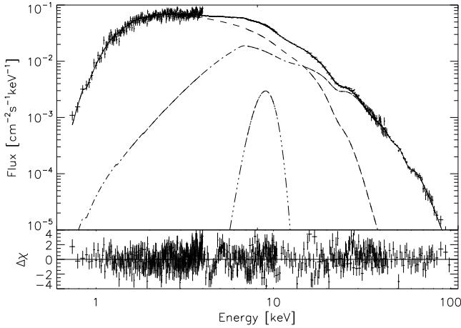
Fig. 4. Upper panel: the unfolded spectrum of 4U 0115+63 described by the Comptonization model: the dashed line is the thermal Comptonization, the dot-dashed line the column emission computed using the BW model, the dot-dot-dashed line a narrow Gaussian line, and the solid line the sum. The spectra of the four instruments have been scaled according to the inter-calibration constants of Table 1. Lower panel: residuals from the best fit model.
