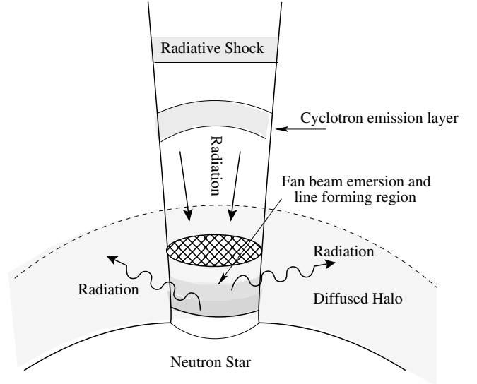
Fig. 11. A schematic and not in scale cartoon of the magnetospheric structure of 4U 0115+63, as it emerges from our analysis.
