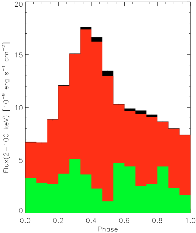
Fig. 10. Contribution of the BW model plotted in red (dark gray), compTT in green (light gray), and the Gaussian emission line in black to the total flux (points with error bars).
