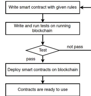
Fig. 6. Smart contracts implementation workflow.
