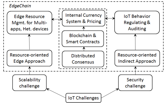
Fig. 2. EdgeChain vision: the problem space and solution space.
