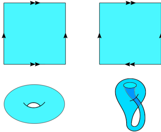
FIGURE 4. A torus \mathbb{T} and a Klein bottle \mathbb{K} , the resulting shapes of two possible identifications of the opposite sides of a plaquette. The left plaquette is a cycle with any field coefficients and the right is only a cycle with \mathbb{F}_2 coefficients.
