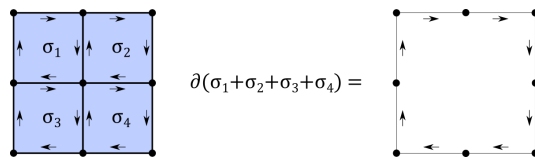
FIGURE 2. The boundary of a union of 4 plaquettes computed with the linearity of the boundary operator.
