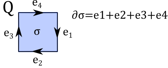
FIGURE 1. The boundary map for a two dimensional plaquette.
