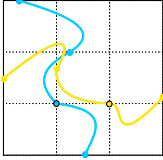
FIGURE 5. The two paths constructed in Lemma 45. The blue path is a projection of a witness for the event H and the yellow path is a projection of a witness for I . The circled blue dot is \mathbf{v} and the circled orange dot is \mathbf{w} . Both paths are shown in \Lambda with a grid spacing of 2n for clarity.
