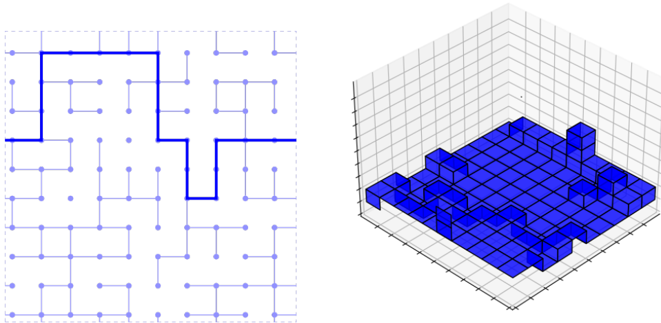
FIGURE 3. Examples of giant cycles: (left) a 1-dimensional giant cycle in \mathbb{T}^2 and (right) a 2-dimensional giant cycle in \mathbb{T}^3 , shown in cubes with periodic boundary conditions. Reproduced with permission from [DKS20].
