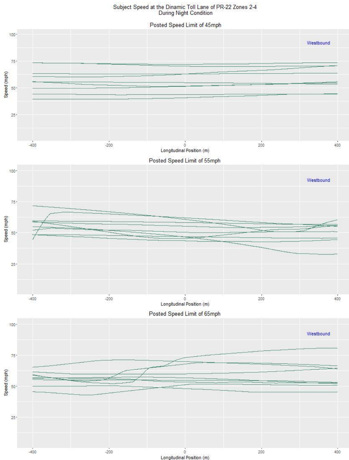
Figure A.6 Subject Speed at the DTL in Zones 2, 3 and 4 During Night Condition for 45, 55 and 65 mph Posted Speed Limit
