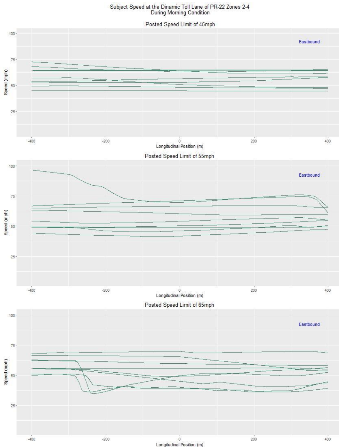
Figure A.4 Subject Speed at the DTL in Zones 2, 3 and 4 During Morning Condition for 45, 55 and 65 mph Posted Speed Limit
