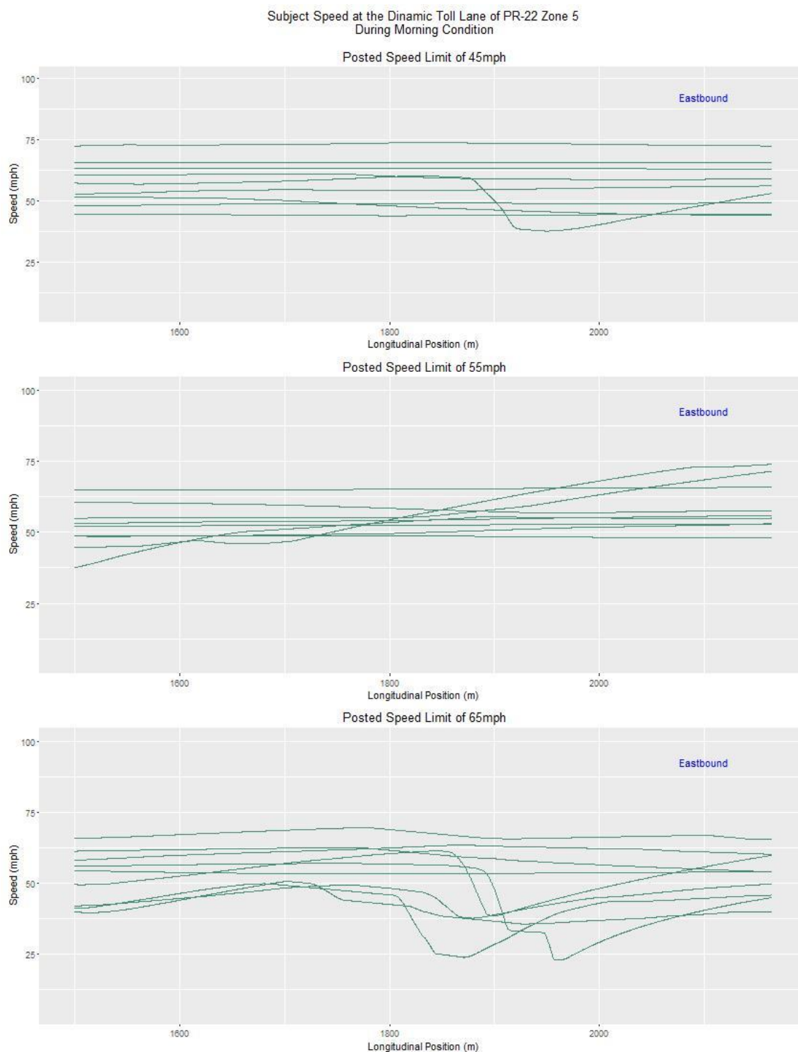
Figure A.7 Subject Speed at the DTL in Zone 5 During Morning Condition for 45, 55 and 65 mph Posted Speed Limit
