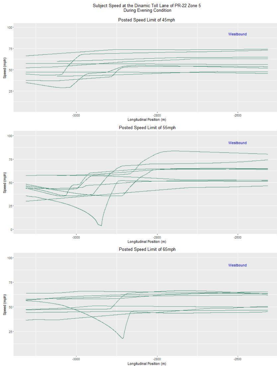
Figure A.8 Subject Speed at the DTL in Zone 5 During Evening Condition for 45, 55 and 65 mph Posted Speed Limit
