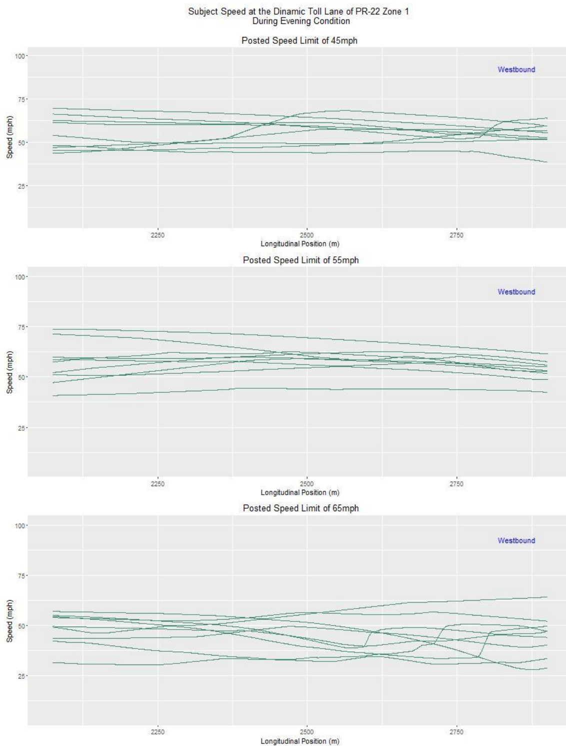
Figure A.2 Subject Speed at the DTL in Zone 1 During Evening Condition for 45, 55 and 65 mph Posted Speed Limit
