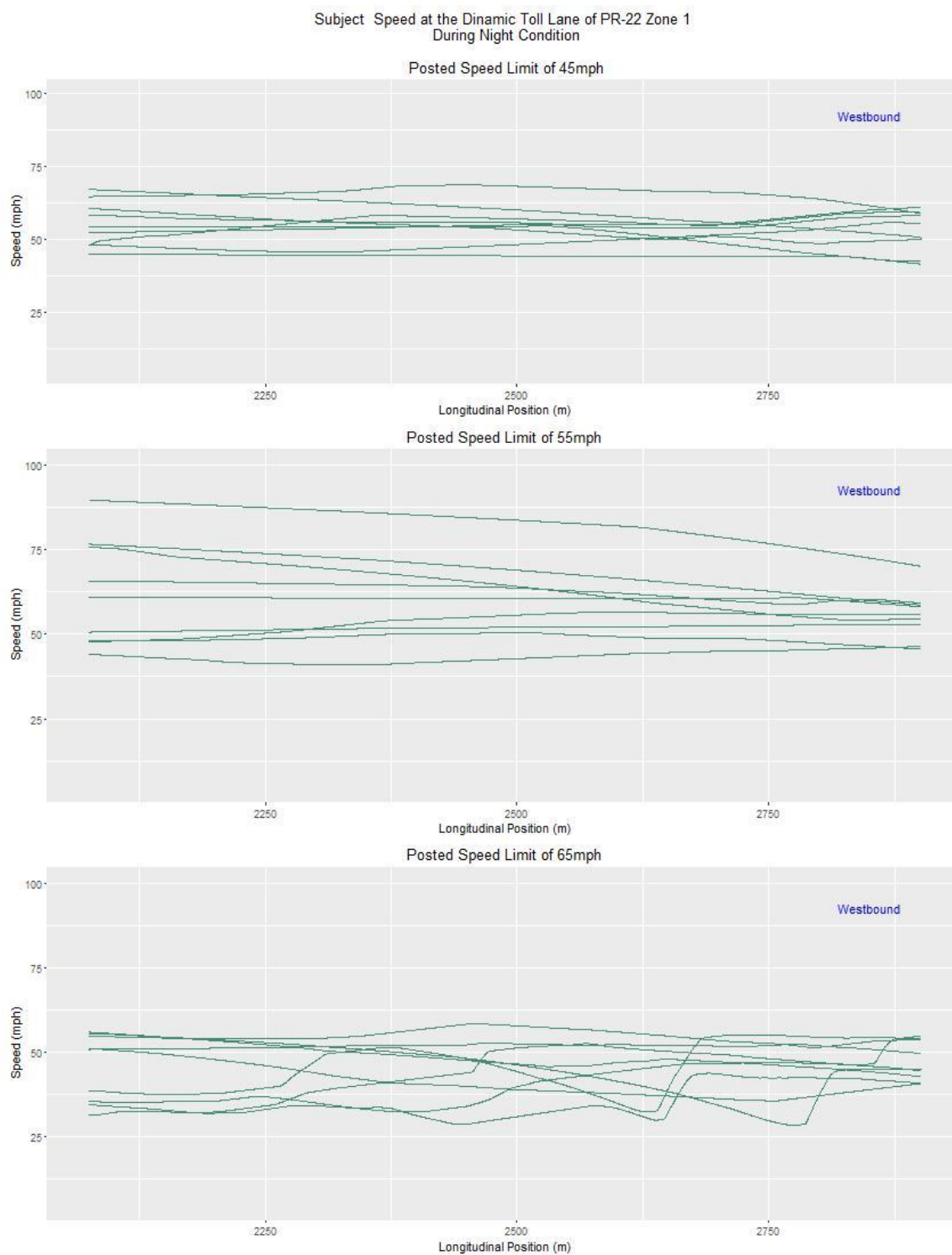
Figure A.3 Subject Speed at the DTL in Zone 1 During Night Condition for 45, 55 and 65 mph Posted Speed Limit
