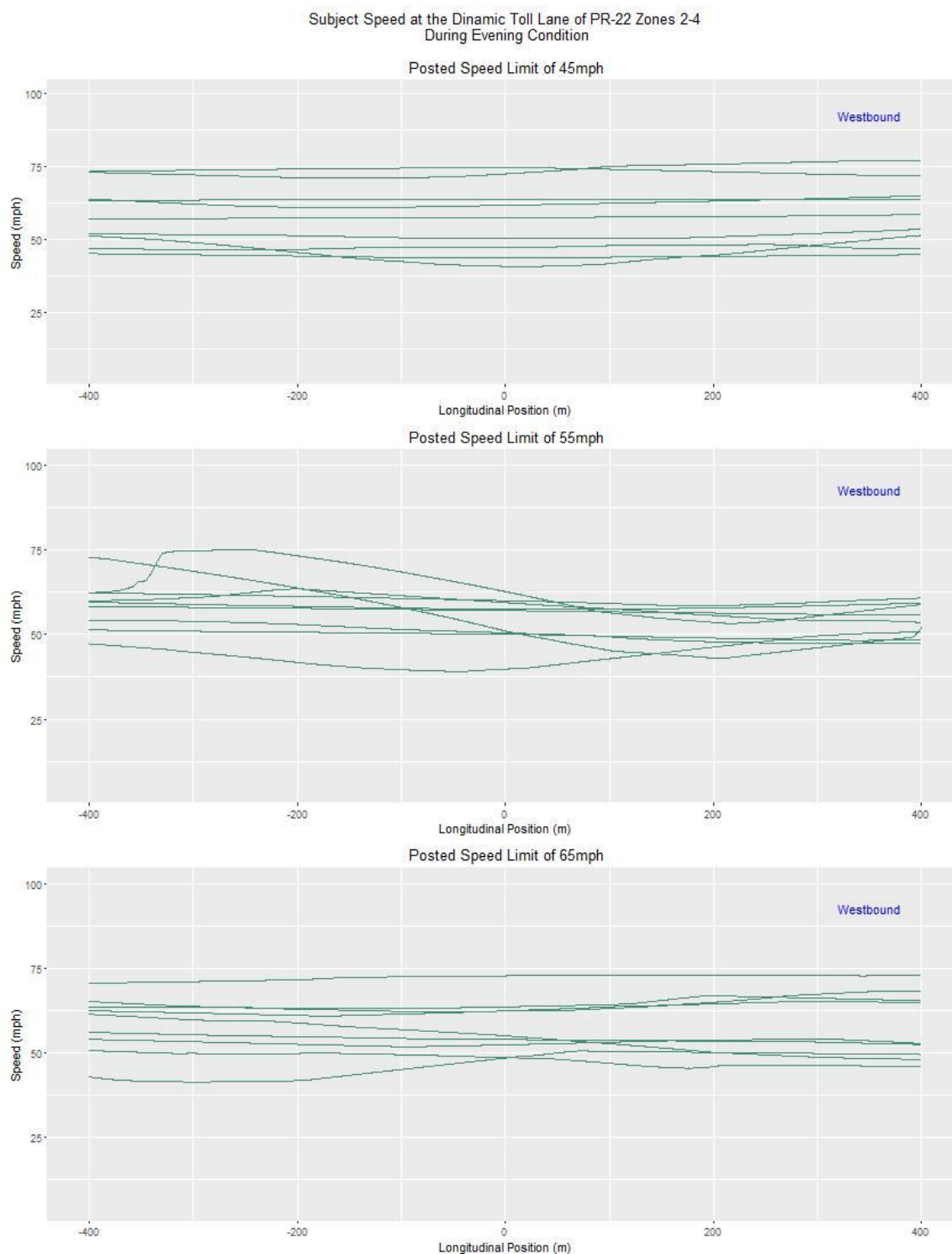
Figure A.5 Subject Speed at the DTL in Zones 2, 3 and 4 During Evening Condition for 45, 55 and 65 mph Posted Speed Limit
