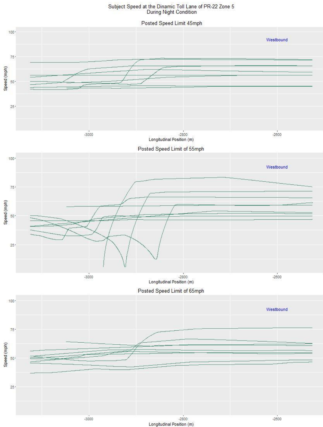
Figure A.9 Subject Speed at the DTL in Zone 5 During Night Condition for 45, 55 and 65 mph Posted Speed Limit
