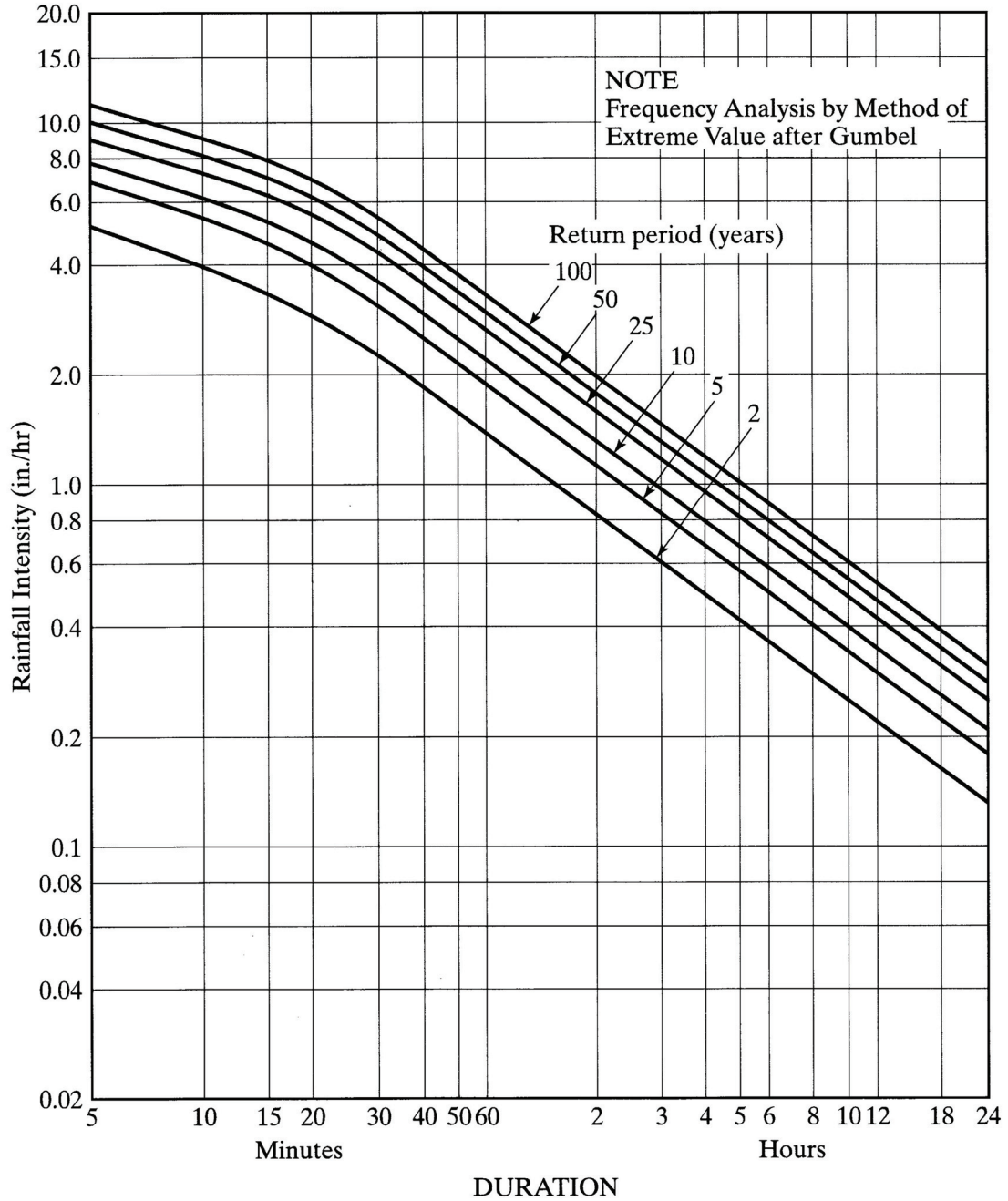
Figure 4.4 Rainfall intensity-duration-frequency (National Weather Service, 1961).
