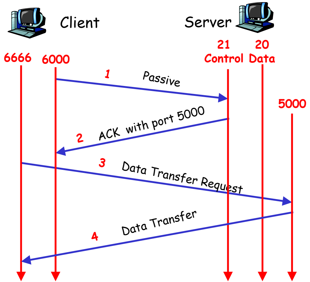
Passive-mode FTP Connection
