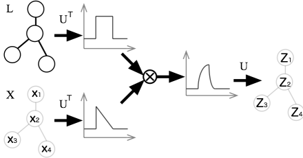
Figure 1: GCN workflow.
