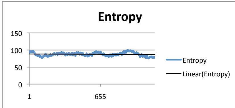
Figure 6. Entropy variation of the session, segment 655 marks the start of the second episode.
