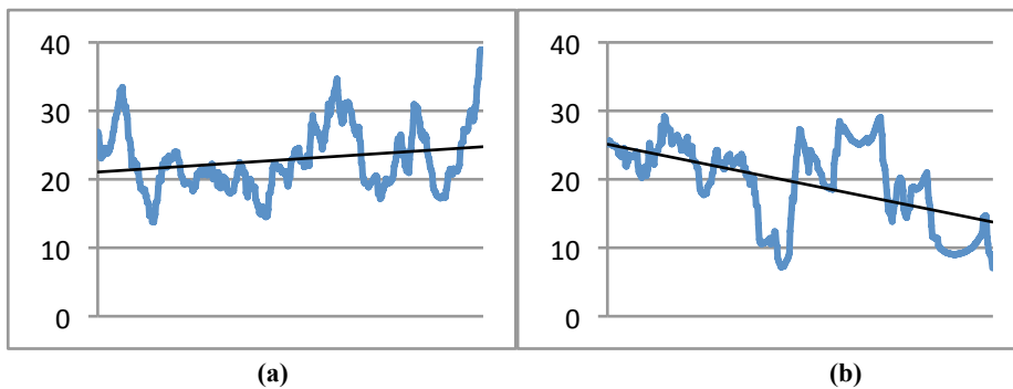
Figure 7. (a) Allan's entropy of the first episode (segment 1 to 526). (b) Allan's entropy of the second episode (segment 655 to 1152)
