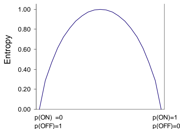
Figure 15. Maximum entropy when p(\text{ON})=p(\text{OFF})=0.5
