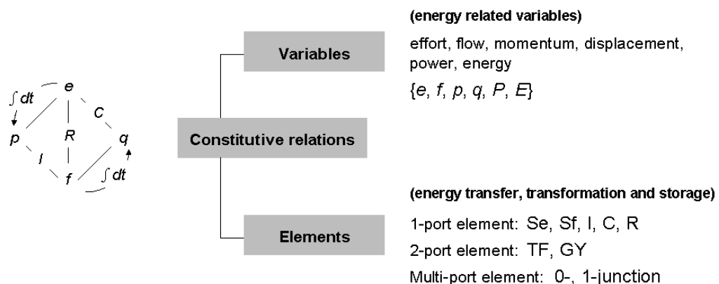
Figure 1 Variables, elements and constitutive relations of bond graphs
