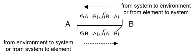
Figure 3 ABG bicausal bond
