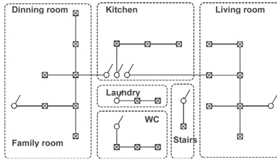
Figure 6 Simplified illumination arrangement plan of townhouse ground floor
