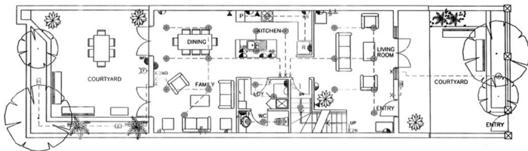
Figure 4 A design drawing of townhouse ground floor plan
