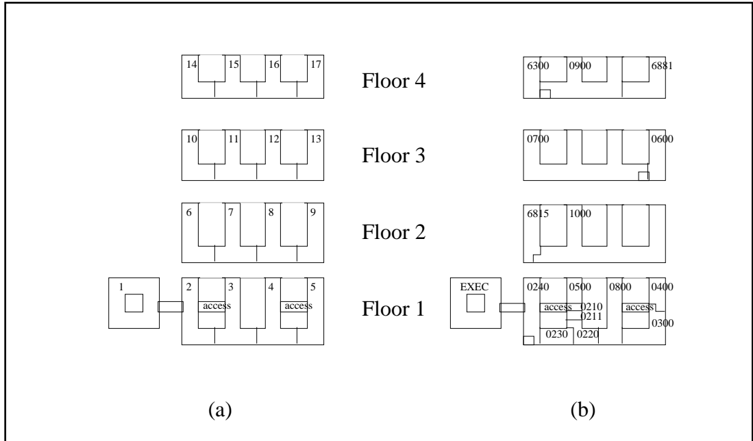
Figure 6 (a) The data defining zones for the office layout problem, and (b) the solution produced by Liggett's system.
