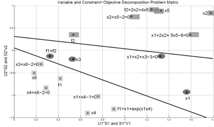
Figure 6: Model-based decomposition using SVD algorithm and K-means clustering
