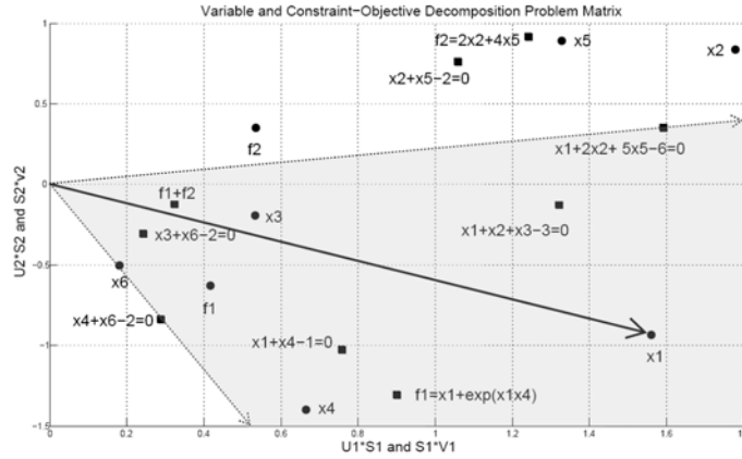
Figure 5: Variables and functions returned with query variable x_1 and cosine similarity threshold of 0.7
