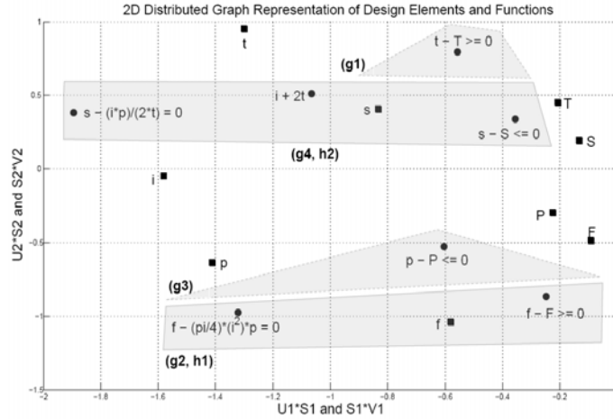
Figure 8: 2D graph of the single objective HCD
