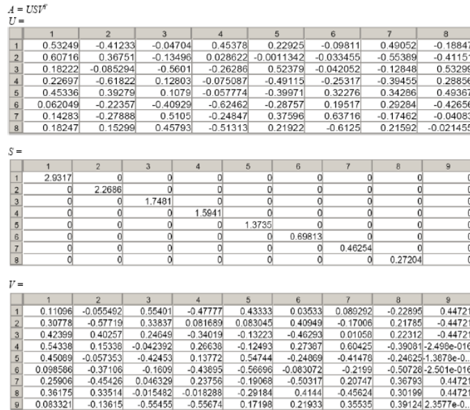
Figure 2: SVD performed on the occurrence matrix A
