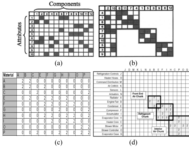
Figure 10: Original incidence matrix problem and (b) its solution; (c) Original DSM and (d) its solution
