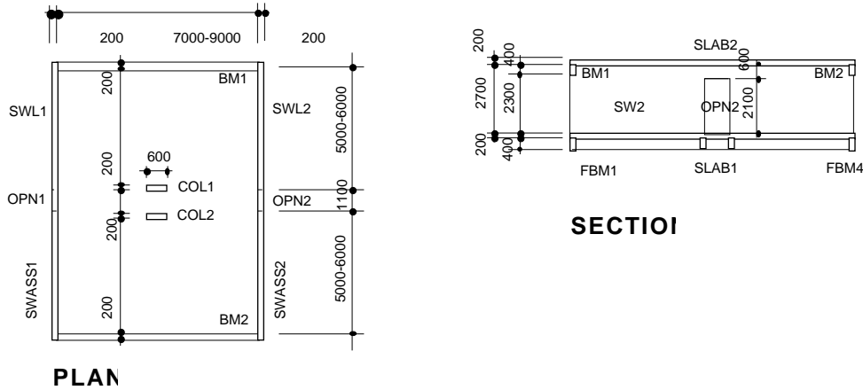
Figure 5. Structural Engineers' Graphical Representation
