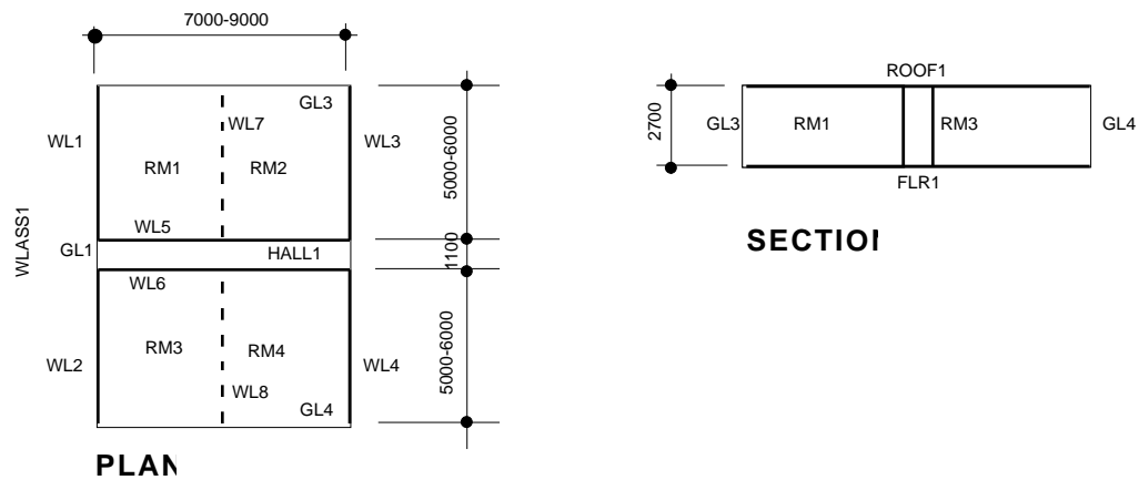
Figure 3. Graphical Representation of Architects' First Concept.
