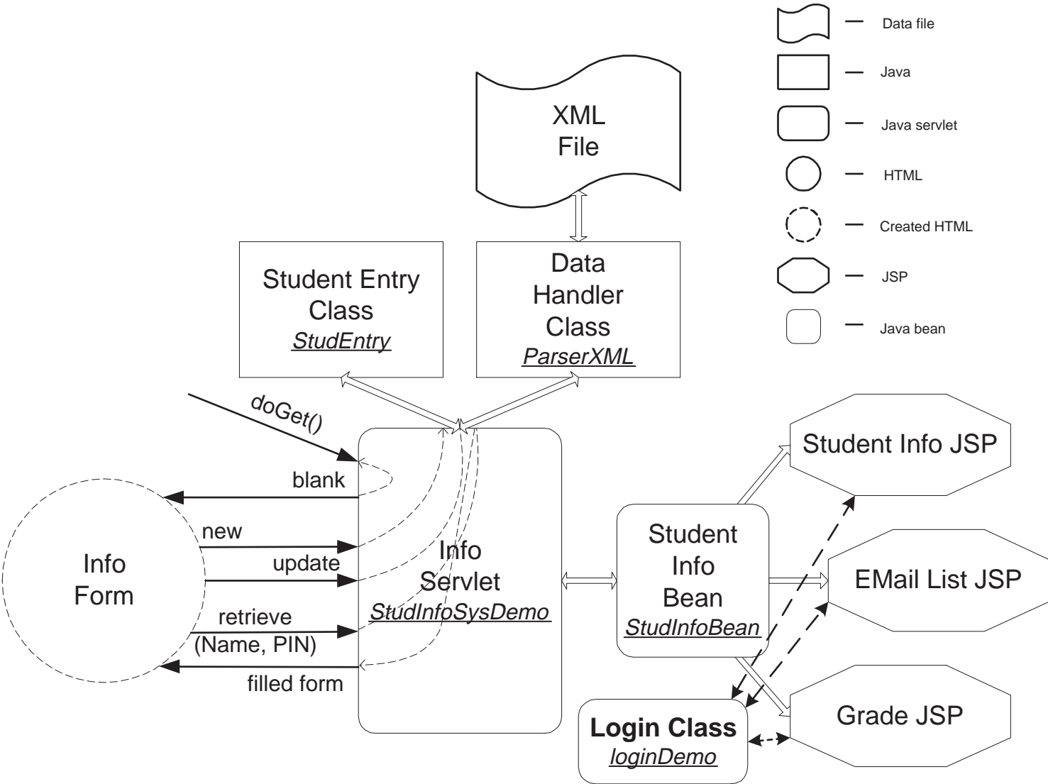
Architectural Design of a Simple Student Information System
