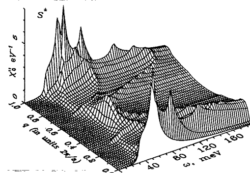
FIG. 3. Renormalized susceptibility \chi''^{(-)}(q_x, q_y, \omega) , plotted as a function of q = q_x = q_y and \omega for the same s^{\pm} state as in Fig. 2.
