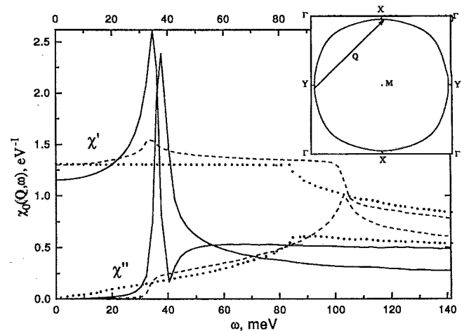
FIG. 1. The imaginary \chi_0^{''(-)}(\mathbf{Q}, \omega) and real \chi_0^{'(-)}(\mathbf{Q}, \omega) parts of the electron spin susceptibility in the superconducting s^\pm (solid and dashed lines) and normal (dots) states at T = 0 . Dashed lines and dots correspond to the Fermi energy \mu = -370 meV, solid lines to \mu = -440 meV. Inset: The Fermi surface for \mu = -440 meV.
