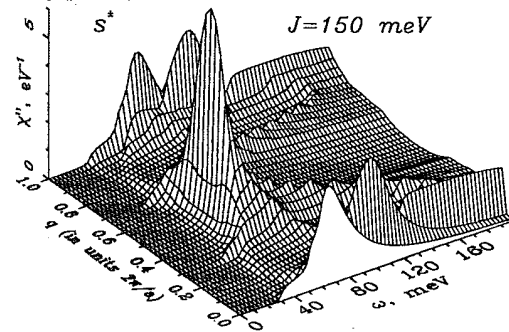
FIG. 2. Bare susceptibility \chi_0^{(-)}(q_x, q_y, \omega) , plotted as a function of q = q_x = q_y and \omega for the s^{\pm} order parameter with \mu = -440 meV.
