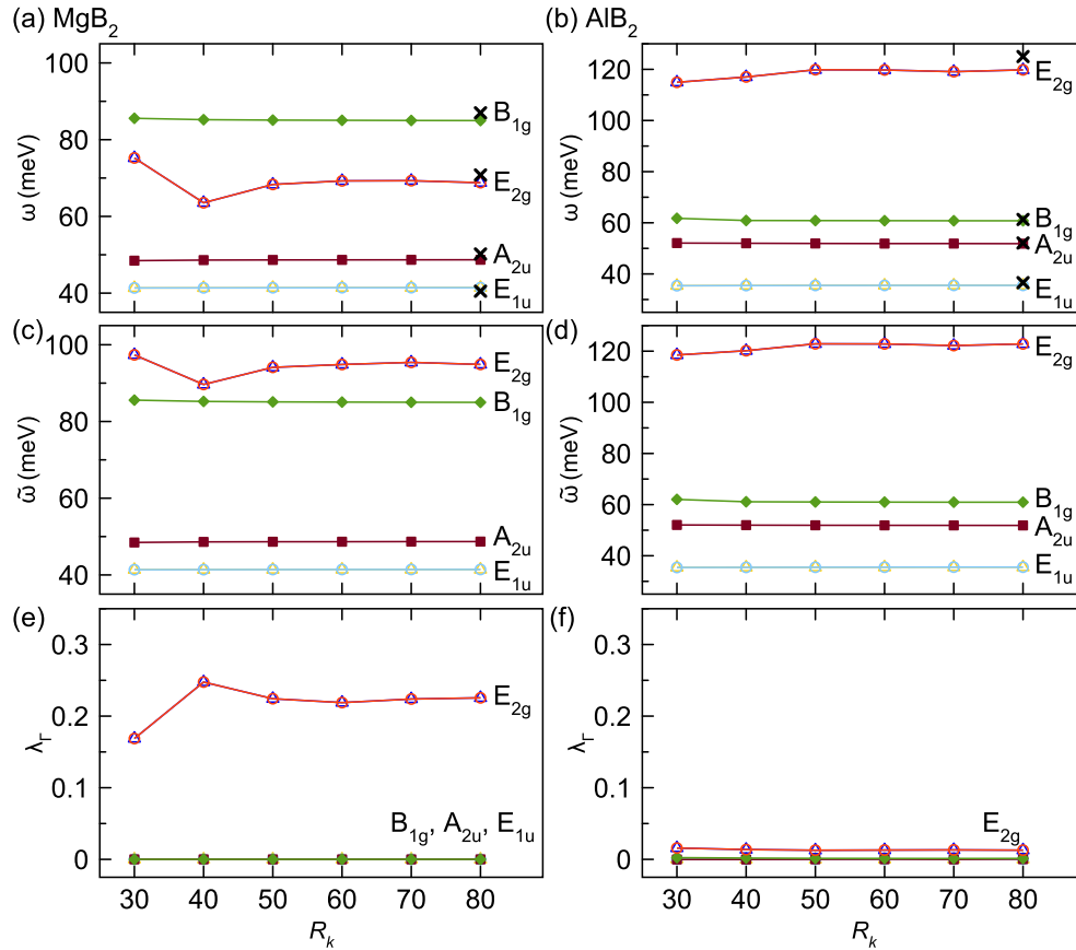
FIG. 2. Zone-center EPC strength calculations for \text{MgB}_2 and \text{AlB}_2 . (a), (b) the screened phonon frequencies \omega . (c), (d) unscreened phonon frequencies \tilde{\omega} . (e), (f) zone-center EPC strength \lambda_\Gamma . R_k is the reciprocal lattice spacing that determines the \mathbf{k} grid density. Each symbol (and color) represents one phonon mode. The two curves representing doubly degenerate E_{2g} and E_{1u} modes are overlapped. The reference data marked by \times in (a) and (b) are from Ref. [29].
