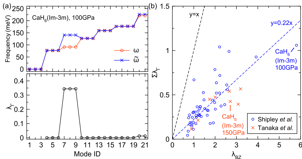
FIG. 3. (a) The screened and unscreened phonon frequencies (top panel) and zone-center EPC strength (bottom panel) in the \text{CaH}_6 ( Im\bar{3}m ) phase at 100 GPa. (b) Scatter plot of zone-center EPC strength \lambda_\Gamma versus EPC constant from full BZ calculations \lambda_{\text{BZ}} for datasets by Tanaka et al. [33] and Shipley et al. [34]. The dashed lines indicate linear relations with different slopes.
