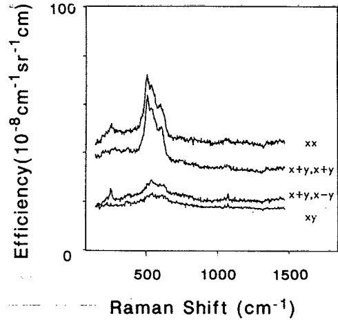
FIG. 3. Raman spectra of a \text{Tl}_2\text{Ba}_2\text{Ca}_2\text{Cu}_3\text{O}_{10} epitaxial film on a \text{MgO} substrate, T_c = 120 K ( \lambda_L = 488 nm, T = 300 K) displayed in absolute units. The electronic Raman cross sections were determined at 1200 \text{cm}^{-1} .
