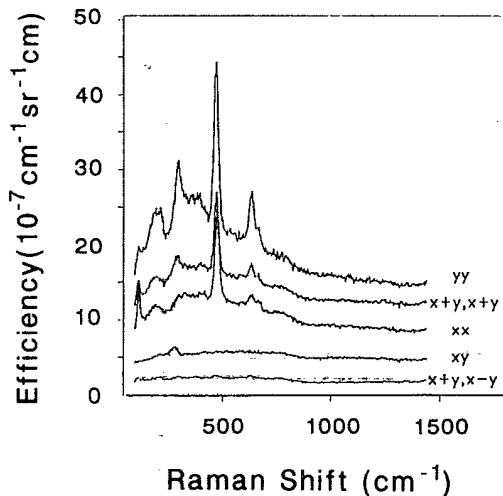
FIG. 2. Raman spectra of a \text{Bi}_2\text{Sr}_2\text{CaCu}_2\text{O}_8 single crystal taken in different polarization geometries at \lambda_L = 488 nm ( T = 300 K). The data are displayed in absolute units with consecutive offsets of (0, 1, 2, \dots, 4) \times 2.5 . The electronic Raman cross sections were determined at 1200 \text{cm}^{-1} .
