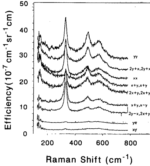
FIG. 1. 300 K Raman spectra of a \text{YBa}_2\text{Cu}_3\text{O}_{7-\delta} single-domain crystal taken with nine different polarizations in the a - b plane at \lambda_L = 514 nm ( T = 300 K). The spectra are displayed in absolute units but include consecutive offsets of (0, 1, 2, \dots, 8) \times 2.5 . The electronic Raman cross sections were determined at a 700 \text{cm}^{-1} frequency shift.
