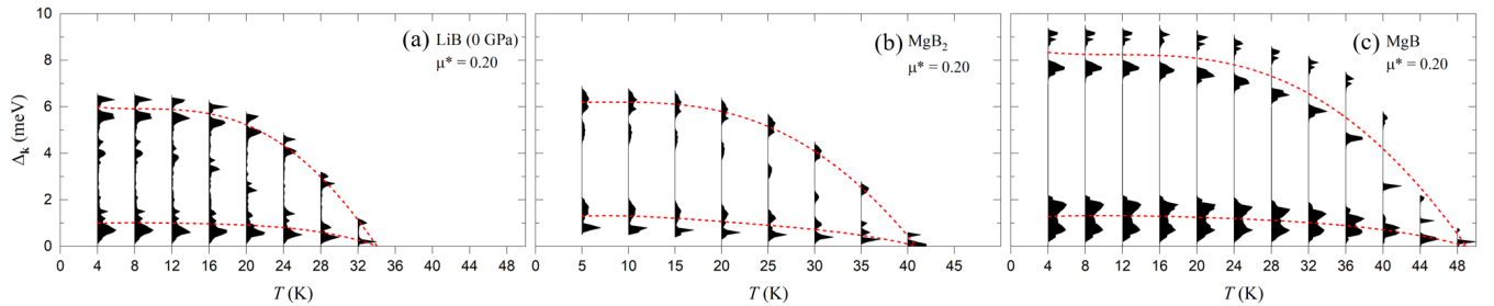
FIG. S4. Calculated anisotropic superconducting gaps \Delta_{\mathbf{k}} of (a) LiB, (b) \text{MgB}_2 , and (c) MgB as a function of temperature with \mu^* = 0.20 . The red dashed curves are a guide to the eye.
