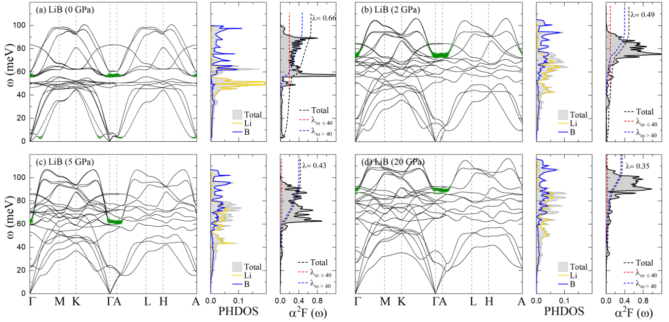
FIG. S7. Calculated phonon dispersion, PHDOS, and Eliashberg spectral function \alpha^2 F(\omega) of LiB at (a) 0, (b) 2, (c) 5, and (d) 20 GPa. The phonon branches are broadened by the e -ph coupling strength \lambda_{\mathbf{q}\nu} , showcasing the modes and high-symmetry directions that have the strongest e -ph coupling.
