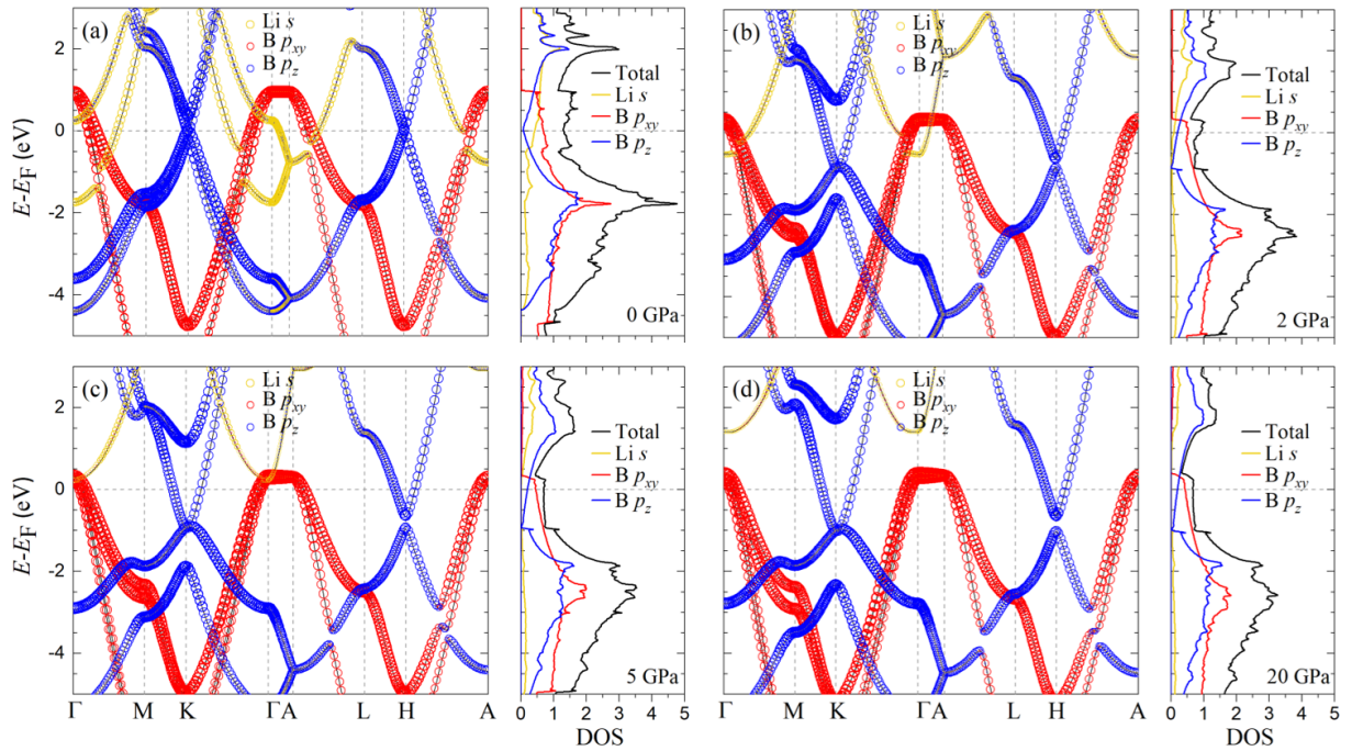
FIG. S6. Calculated band structure and DOS [states/(eV f.u.)] of LiB at (a) 0, (b) 2, (c) 5, and (d) 20 GPa. The size of the symbols is proportional to the contribution of each orbital character.
