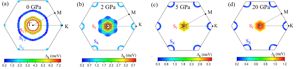
FIG. S8. The distribution of superconducting gap at 4 K on the cross-section Fermi surface plane through z=0 of LiB at (a) 0, (b) 2, (c) 5, and (d) 20 GPa.
