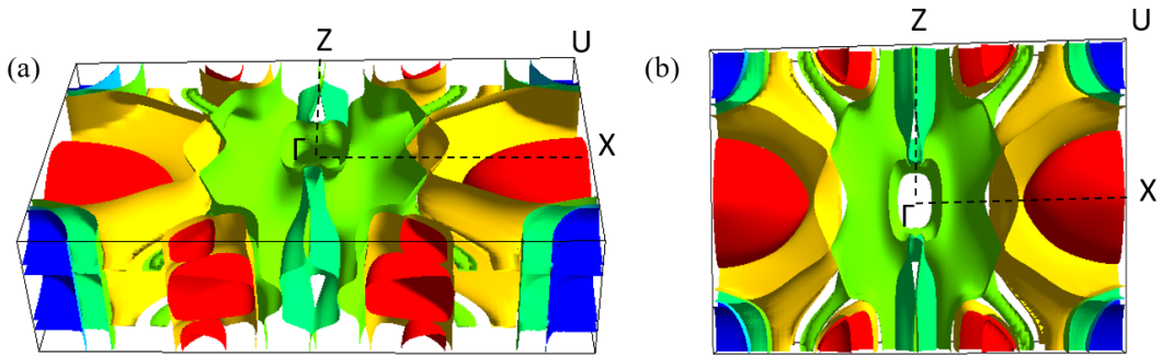
FIG. S14. (a) Side and (b) top view of the Fermi surface of LiMgB 2 .
