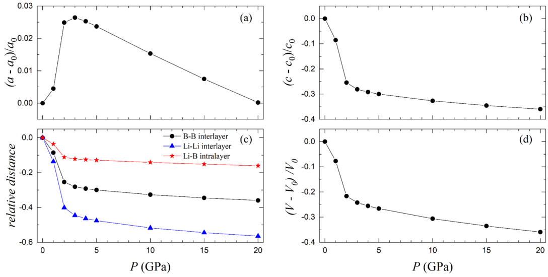
FIG. S5. Pressure dependence of the relative change of (a)-(b) lattice parameters a and c , (c) B-B interlayer, Li-Li interlayer, and Li-B intralayer distances, and (d) volume per formula unit of LiB.
