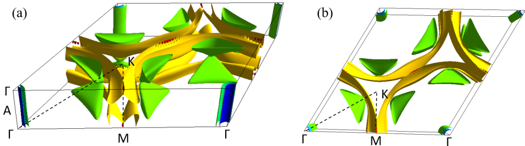
FIG. S13. (a) Side and (b) top view of the Fermi surface of MgB.
