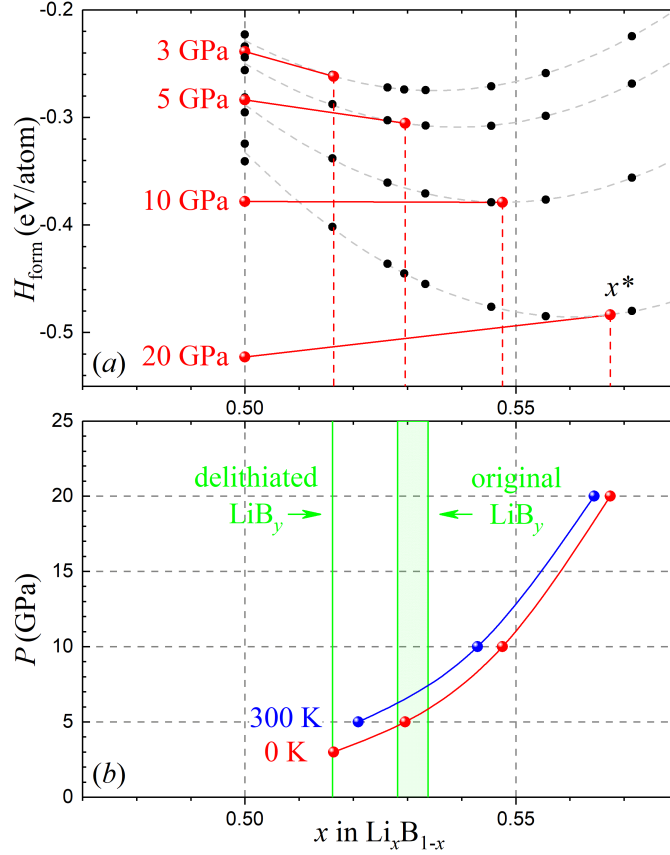
FIG. S1. Analysis of the \text{LiB}_y stability with respect to decomposition into LiB and \text{LiB}_{y^*} ( y^* < y ) at zero temperature and different pressures. (a) Fitted parabolas (dashed grey lines) of \text{LiB}_y formation enthalpies (black circles) with tangents (solid red lines) connecting the formation enthalpies of LiB (large red circles). (b) The pressure-dependent concentrations x^* = (1+y^*)^{-1} that define the products of the \text{LiB}_y \Rightarrow \text{LiB} + \text{LiB}_{y^*} decomposition at 0 K (red points) and 300 K (blue points). The 300 K results were obtained via shifting the LiB formation enthalpies in (a) by the difference in the vibrational entropy corrections between the layered LiB and the most stable 1:1 member of the \text{LiB}_y family. The shaded green range marks stable compositions for \text{LiB}_y , while the single green line corresponds to the proposed metastable delithiated \text{LiB}_y with y=15/16 .
