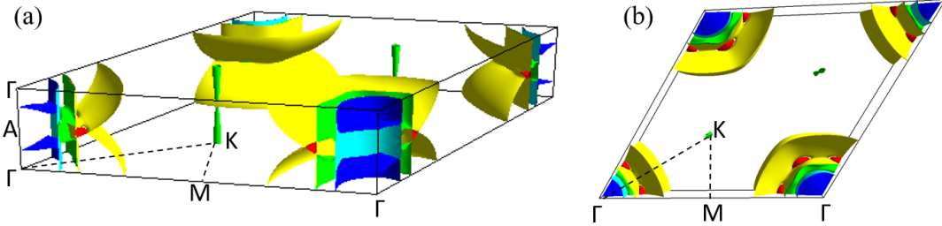
FIG. S3. (a) Side and (b) top view of the Fermi surface of LiB at 0 GPa.
