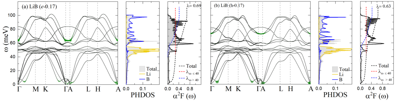
FIG. S11. Calculated phonon dispersion, PHDOS, and Eliashberg spectral function \alpha^2F(\omega) of LiB for the doping level of (a) e -0.17, and (b) h -0.17. The phonon branches are broadened by the e -ph coupling strength \lambda_{q\nu} , showcasing the modes and directions that have the strongest e -ph coupling.
