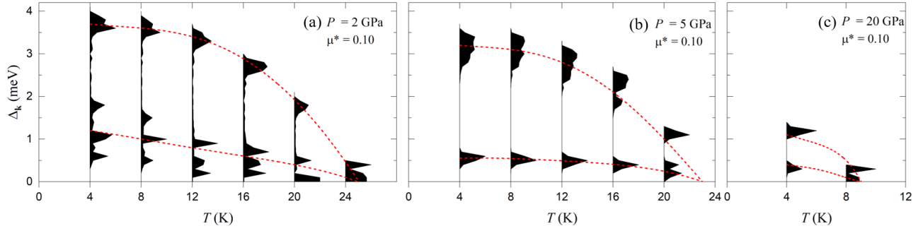
FIG. S9. Calculated anisotropic superconducting gaps \Delta_k of LiB as a function of temperature at (a) 2, (b) 5, and (c) 20 GPa with \mu^* = 0.10 . The red dashed curves are a guide to the eye.
