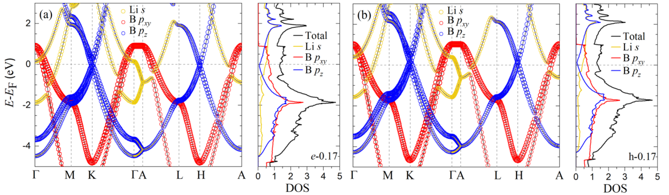
FIG. S10. Calculated band structure and DOS [states/(eV f.u.)] of LiB for the doping level of (a) e-0.17 , and (b) h-0.17 . The size of the symbols is proportional to the contribution of each orbital character.
