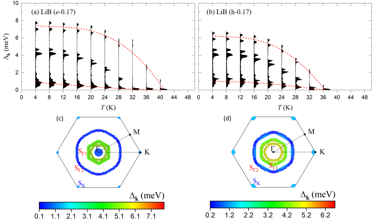
FIG. S12. Calculated anisotropic superconducting gaps \Delta_{\mathbf{k}} of LiB as a function of temperature under (a) e -0.17 and (b) h -0.17 doping with \mu^* = 0.10 . The red dashed curves are a guide to the eye. The distribution of superconducting gap at 4 K on the cross-section Fermi surface plane through z=0 under (c) e -0.17 and (d) h -0.17 doping.
