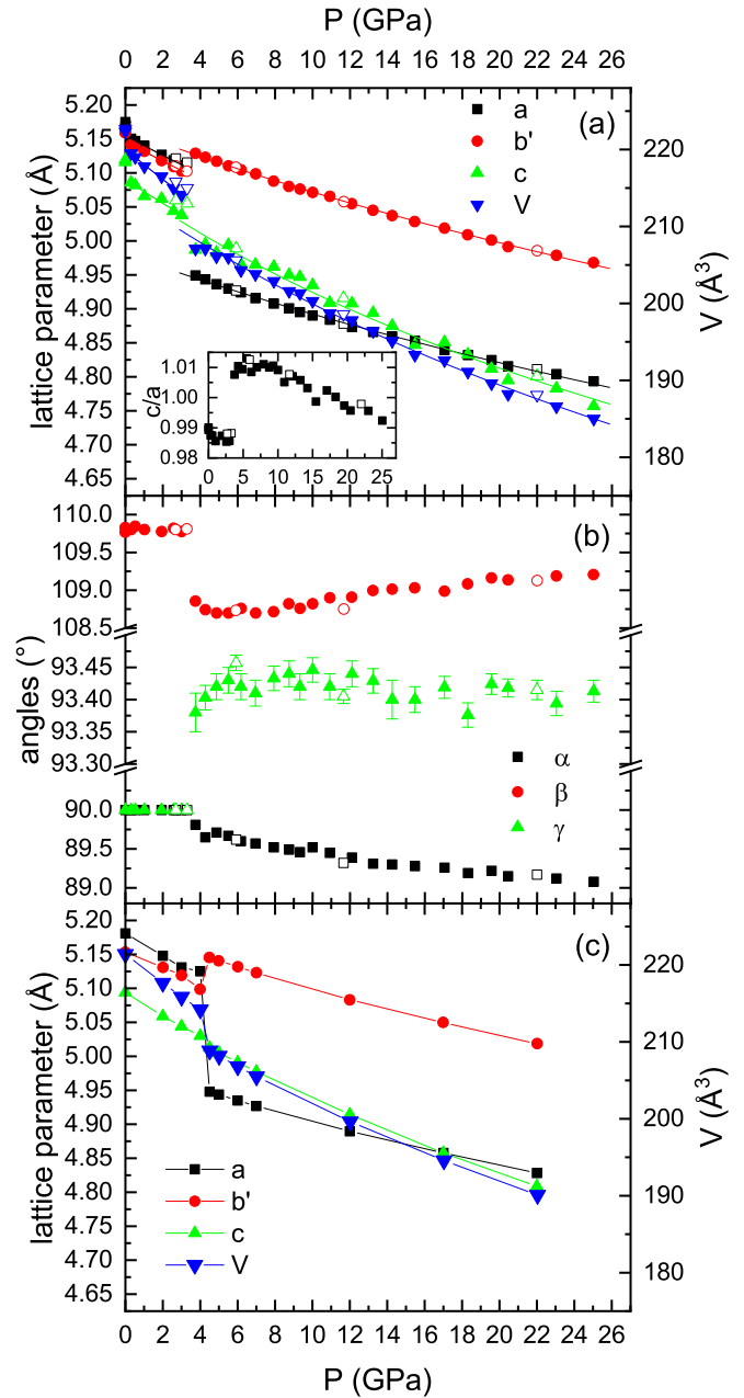
FIG. 1. Pressure dependence of the volume V of the unit cell and the lattice parameters a , b' = b/\sqrt{3} , c , and c/a value shown in (a) and the corresponding angles \alpha , \beta , and \gamma in (b). For a better comparison a nonprimitive unit cell was used for the high-pressure phase above 3.8 GPa, as explained in the text. The solid lines in (a) are fits with a Murnaghan-type equation of state (see text). Open symbols are values observed during pressure release. If not shown, the error bar is smaller than the symbol size. (c) Calculated lattice parameters for pressures up to 22 GPa (corrected by 3 GPa to closely resemble the experimental crystal volume at zero pressure).
