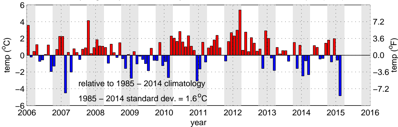
Monthly Temperature Anomaly
