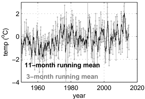
Monthly Temperature Anomaly
