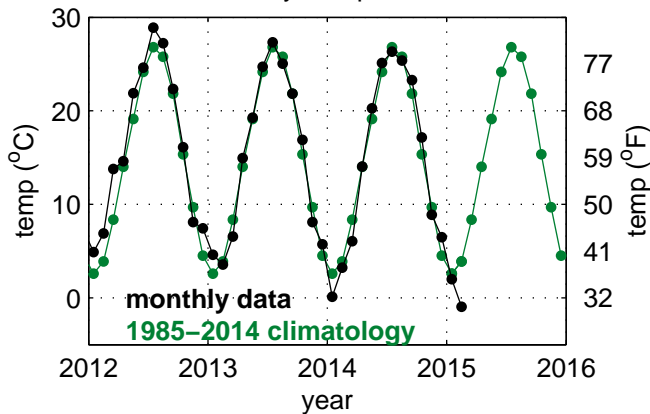
Monthly Temperature
