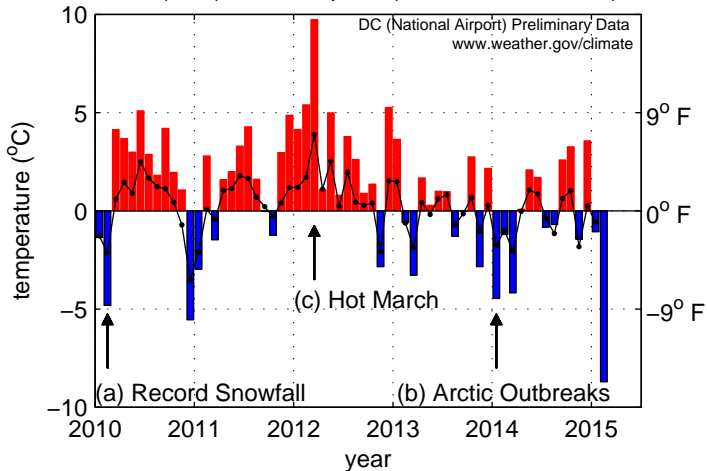
Monthly Avg T (Anomaly from 1985–2014 Avg)
