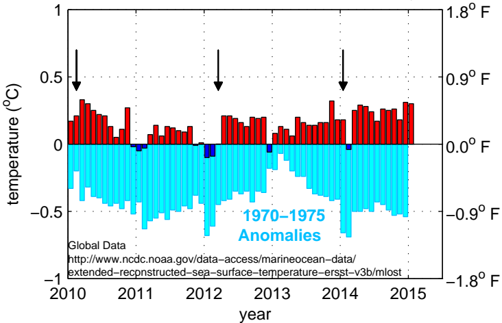
Global Mean Surface Temperature Anomaly
