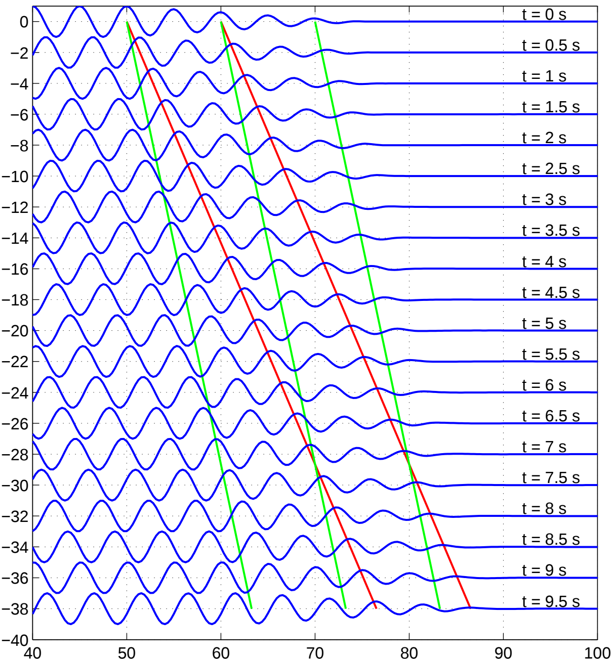
Propagation of short wave group, \lambda = 5 m
