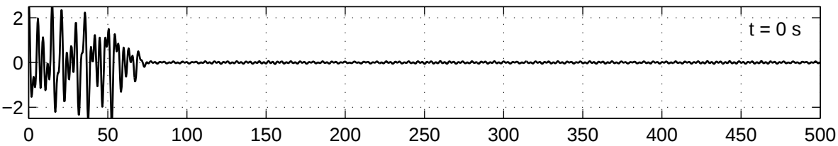
short gravity waves, \lambda = 3 \ 5 \ 7 \text{ m}
