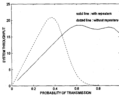
Figure 4 – Throughput of the new structure in comparison to the standard case of not using repeaters in the structure. System parameters are K_c = 30, \lambda_t = 5, R_0 = 1/2, R_1 = 2 .
