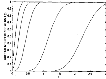
Figure 2 – Cumulative density function for interference at BS due to transmission of all terminals in layer 1. \lambda_I = 5, R_0 = 2/3, R_1 = 2, p_t = .05, .1, .2, .5, 1 which curves to right are related to higher p_t .
